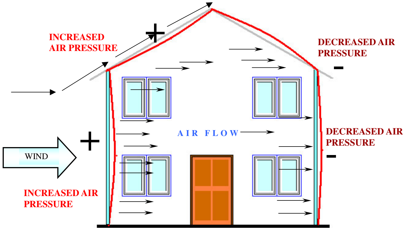
WIND DRIVEN PRESSURE DIFFERENTIAL HIGH SLOPE RAFTERS
