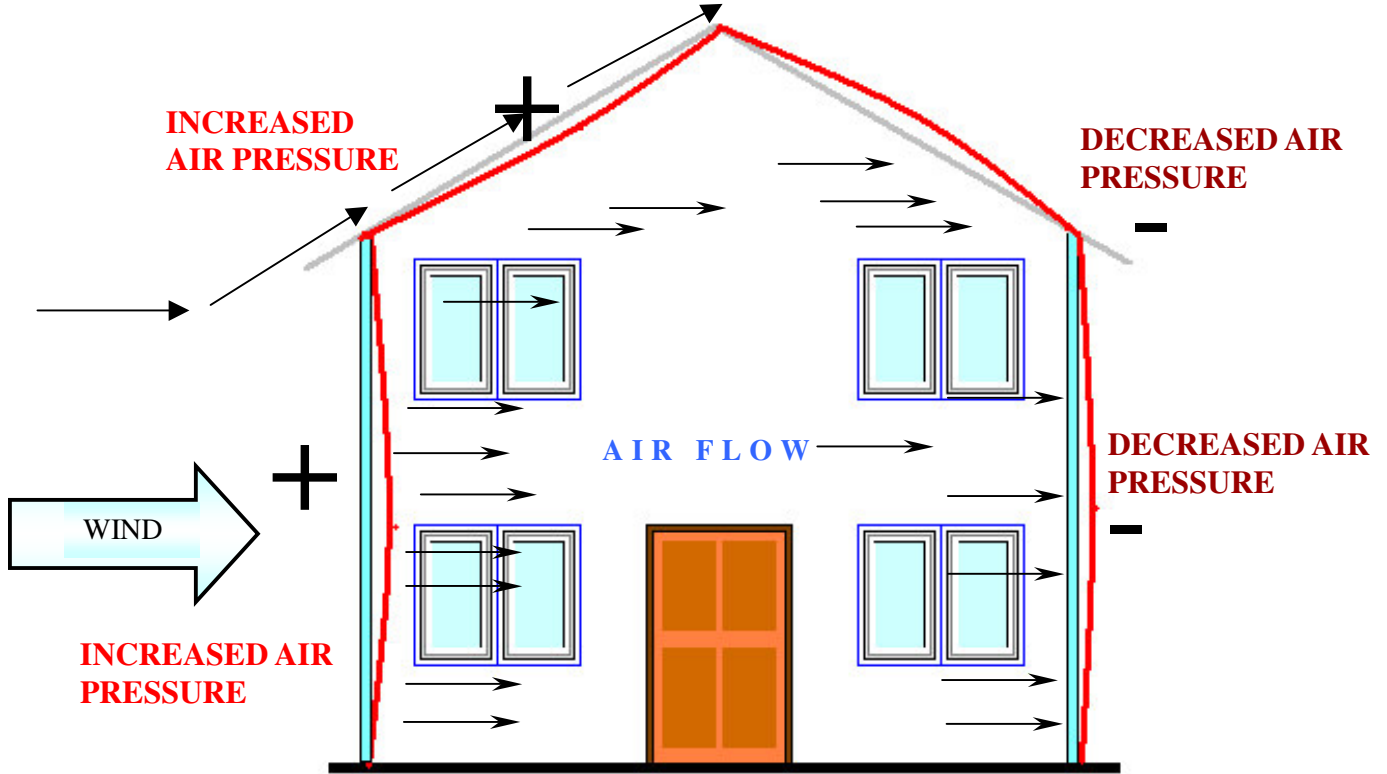
WIND DRIVEN PRESSURE DIFFERENTIAL HIGH SLOPE RAFTERS
